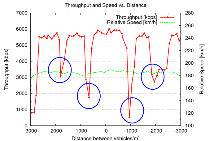
Figure 6. Throughput for the interurban scenario (180 Km/h).
